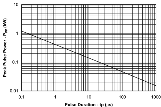
Figure 3. Non-Repetitive Peak Pulse Power vs. Pulse Time
