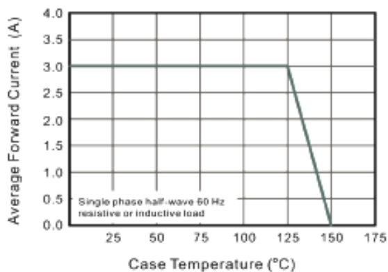
Fig.1 Maximum Average Forward Current Rating
